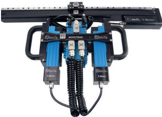
3-Axis - Remote corrosion mapping
